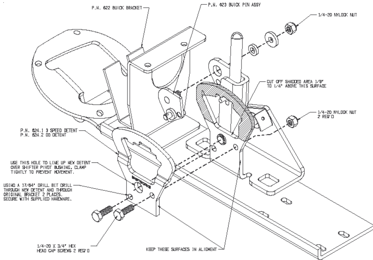
1964-65 BUICK SHIFTER CONVERSION FROM ROD TO CABLE TYPE
